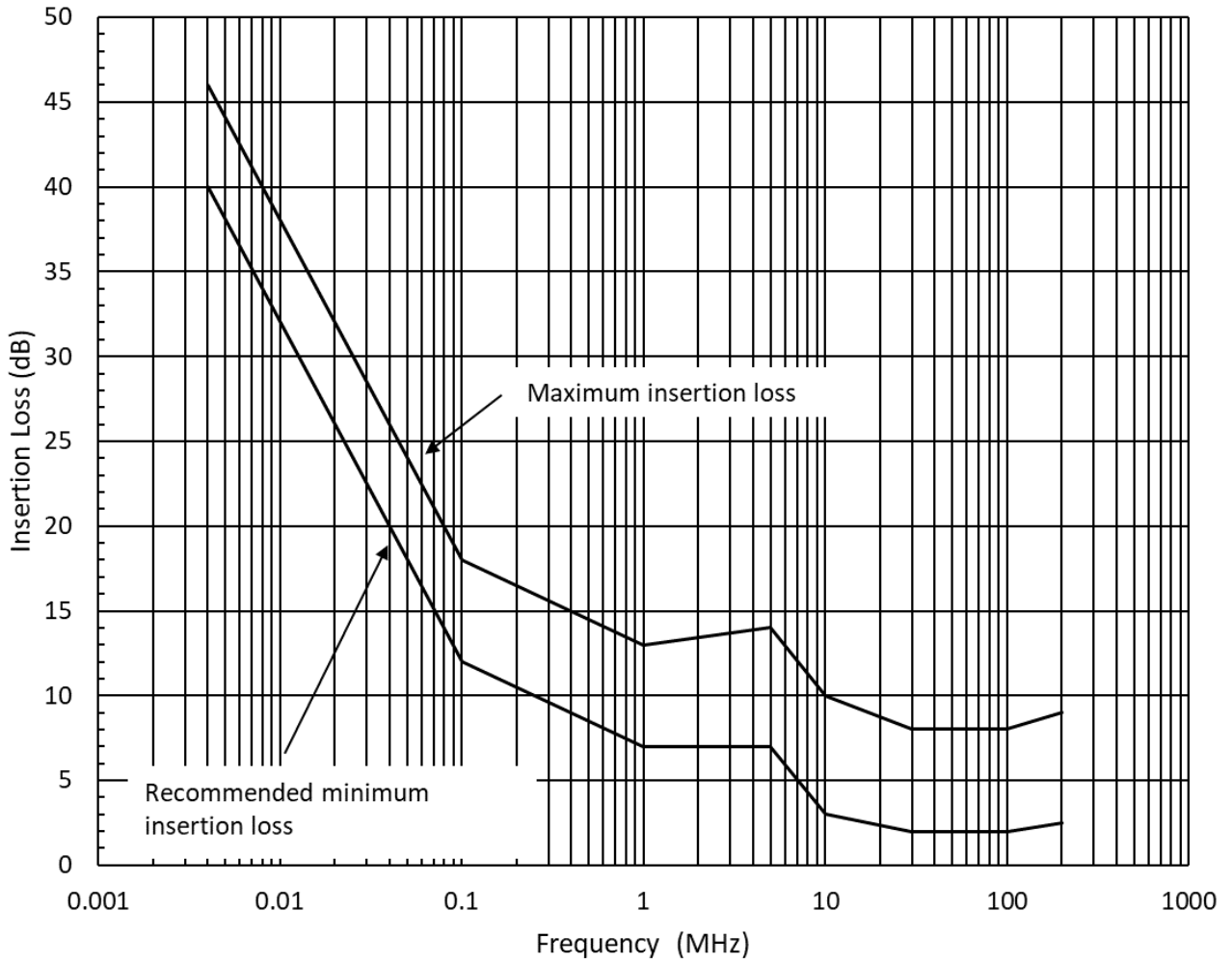
FIGURE CS114- 2. Insertion loss for injection probes.
