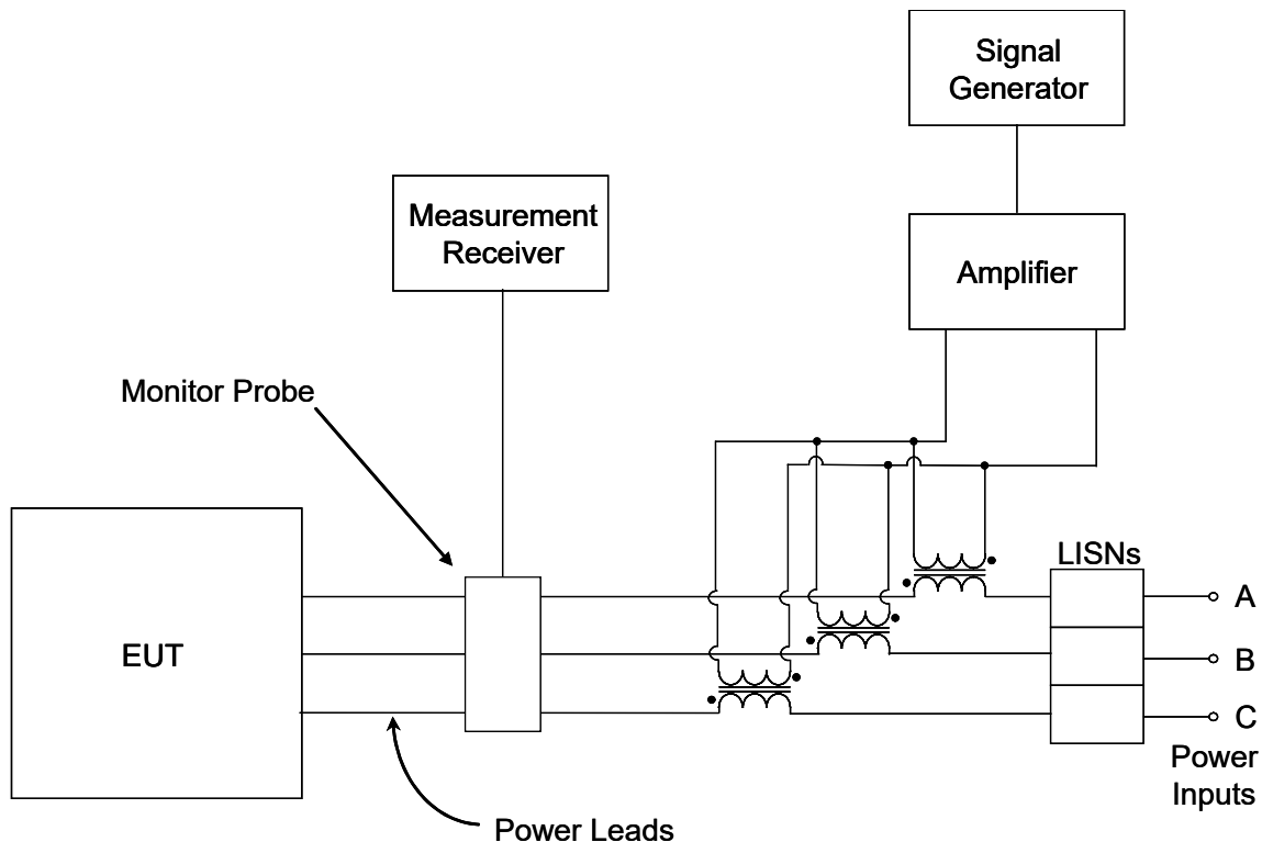
FIGURE A- 20. CS114 alternate test setup, three phase delta power system.
