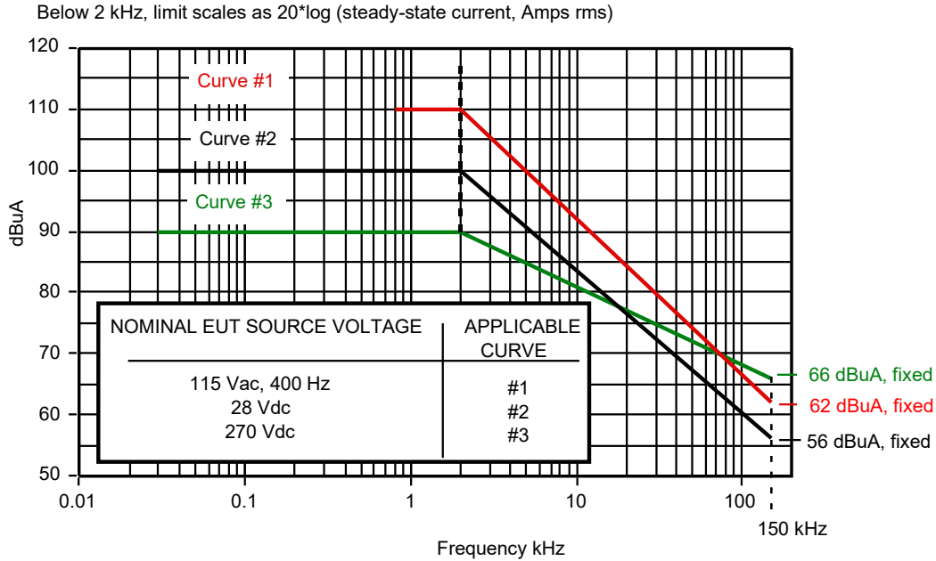
FIGURE A- 10. CE101 limits for a 5 \mu H LISN.
