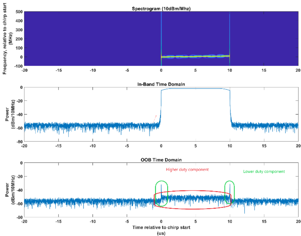
FIGURE A- 28. Example radar pulse characteristics.
