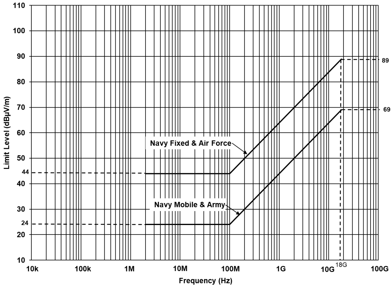
FIGURE RE102- 4. RE102 limit for ground applications.
