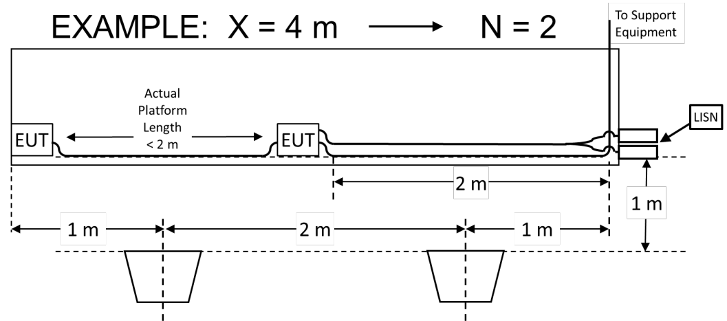
FIGURE RE102- 7. Multiple antenna positions.
