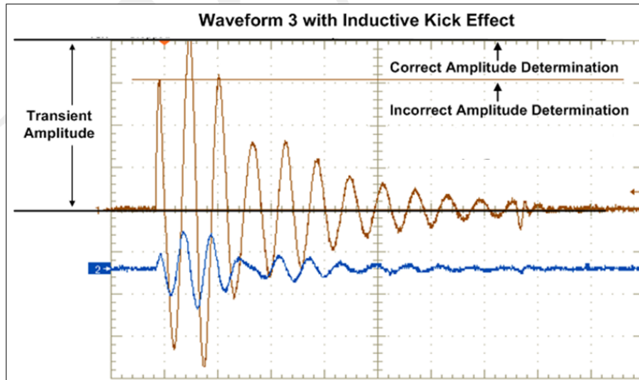
FIGURE A- 27. Inductive kick effect - Waveform 3 amplitude determination.
