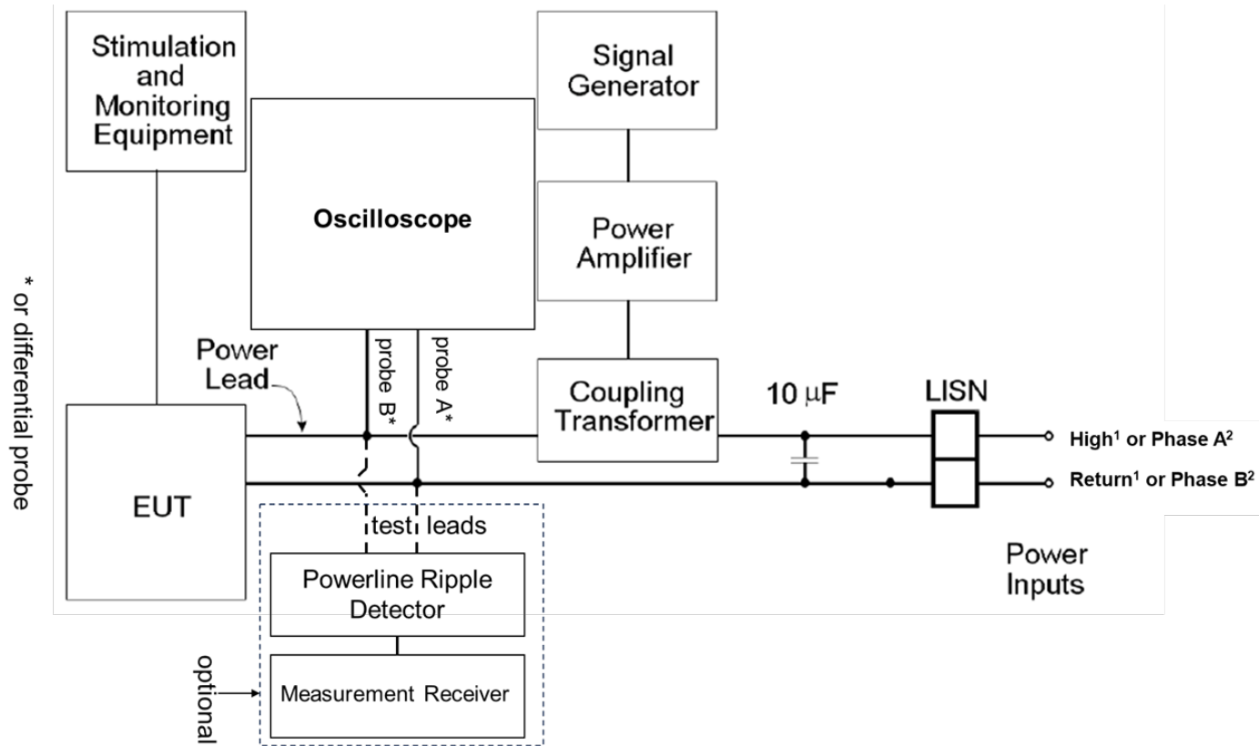
FIGURE CS101- 4. Signal injection, DC 1 or AC (EUT connected to single phase of a wye configured power bus 1 or EUT connected to two phases of a delta configured power bus 2 ).
