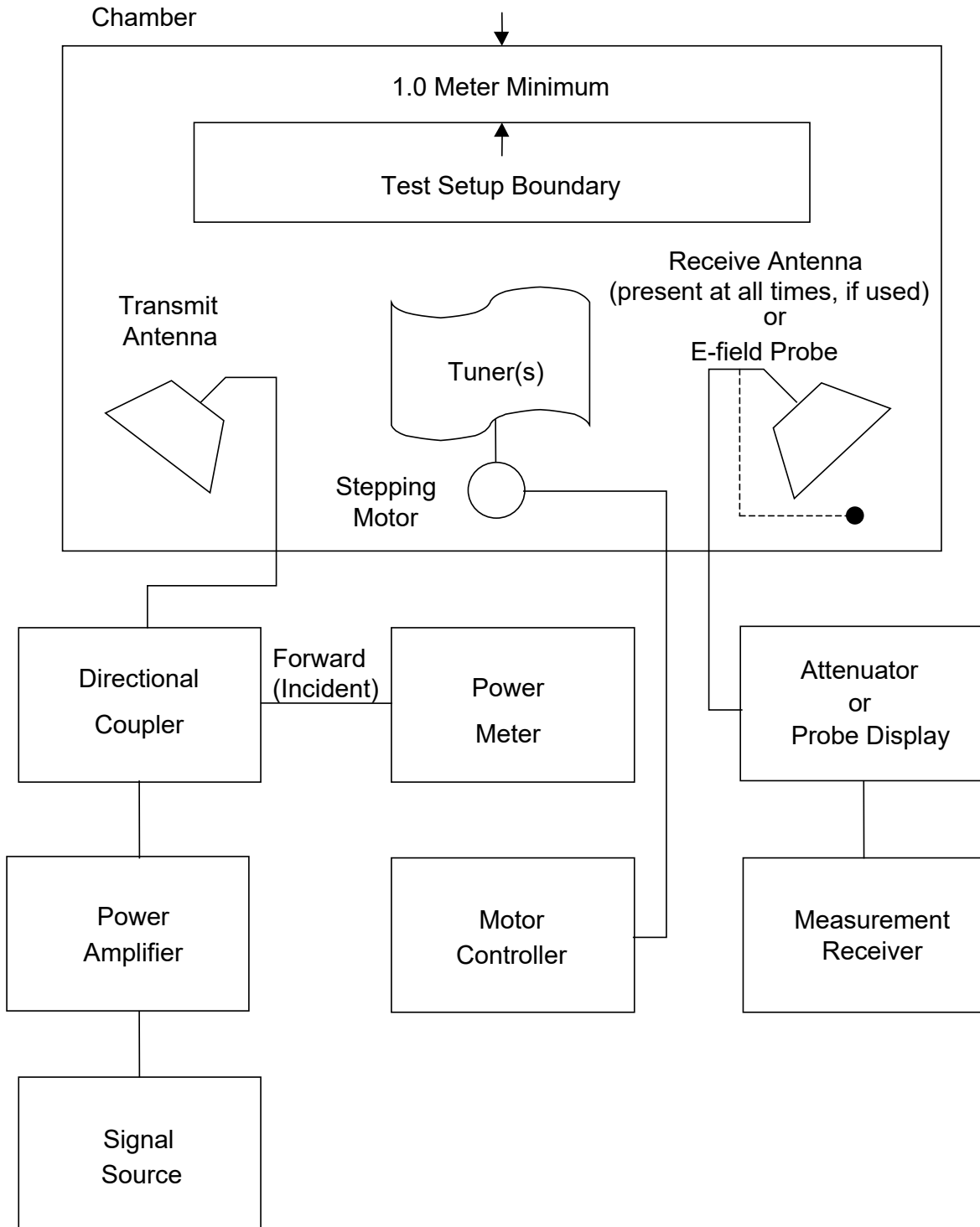
FIGURE RS103- 4. Reverberation chamber setup.
