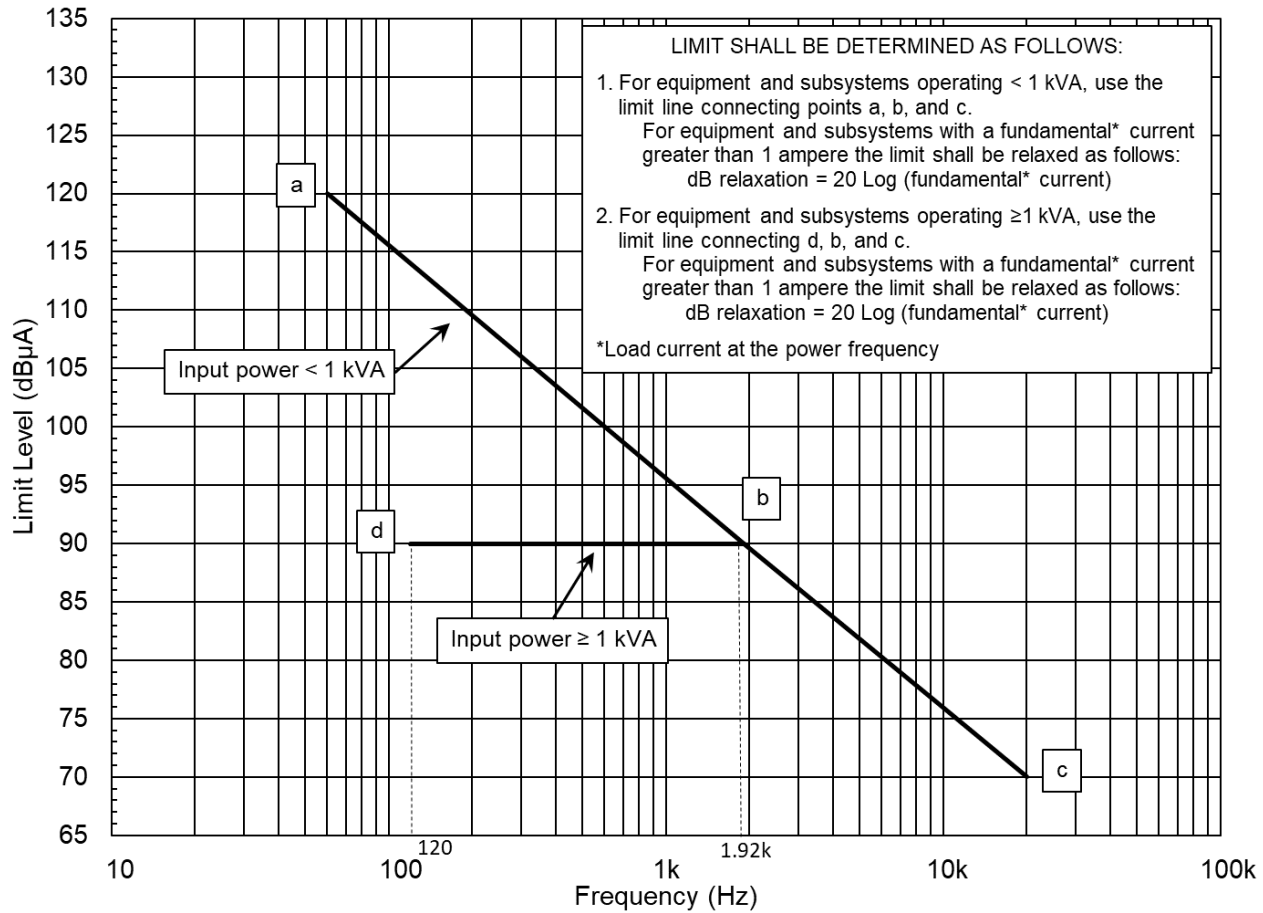
FIGURE CE101- 2. CE101 limit for surface ships and submarine applications, 60 Hz.
