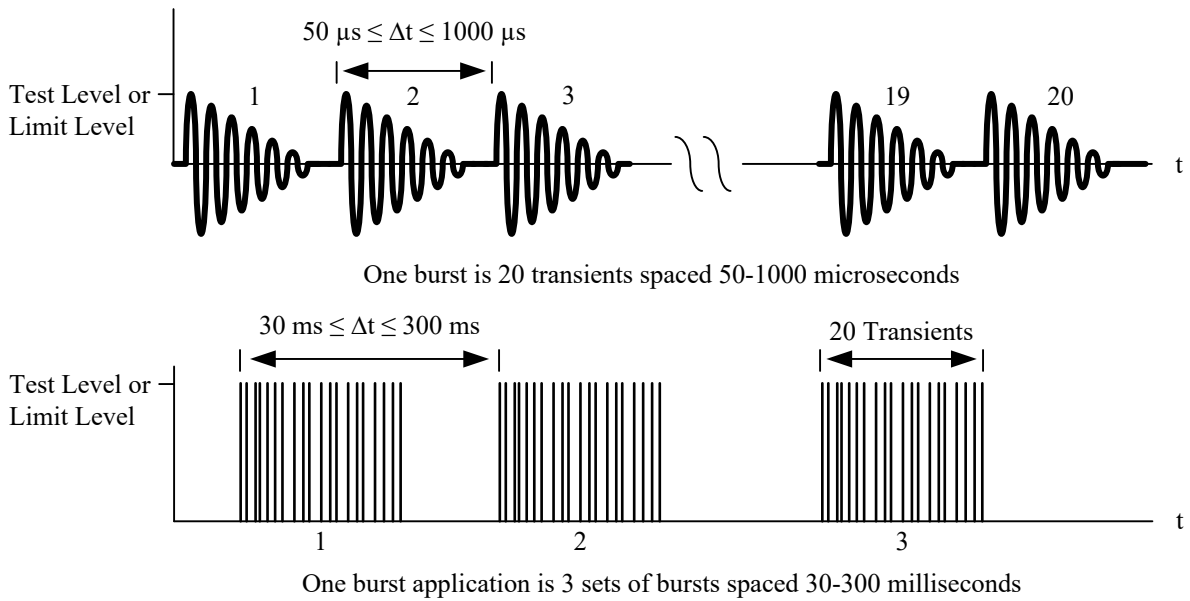
FIGURE CS117- 8. Multiple burst application.
