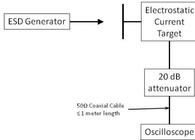
FIGURE CS118- 6. Measurement system check setup, discharge current verification.
