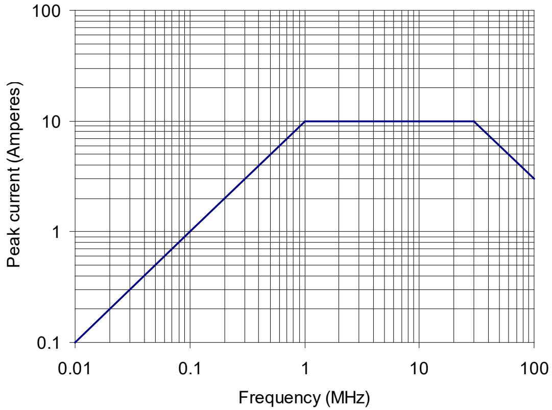
FIGURE CS116- 2. CS116 limit for all applications.
