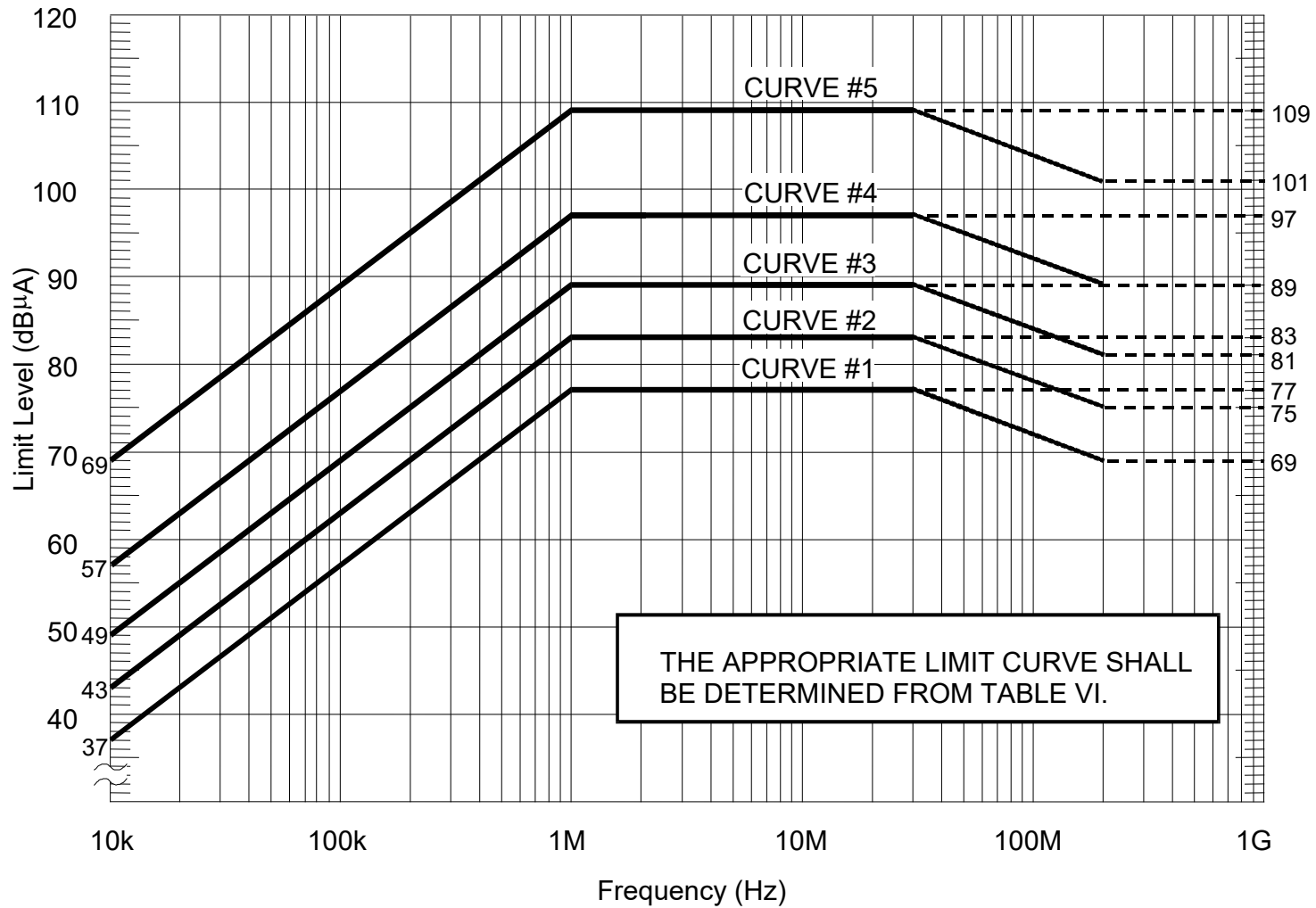
FIGURE CS114- 1. CS114 calibration limits.
