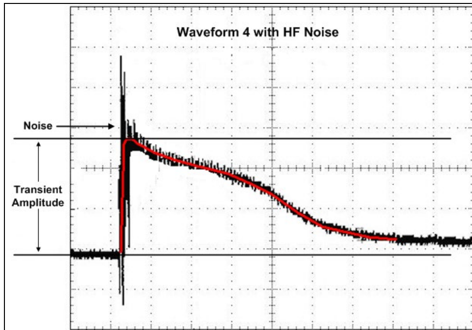
FIGURE A- 25. High frequency noise - Waveform 4 amplitude determination.
