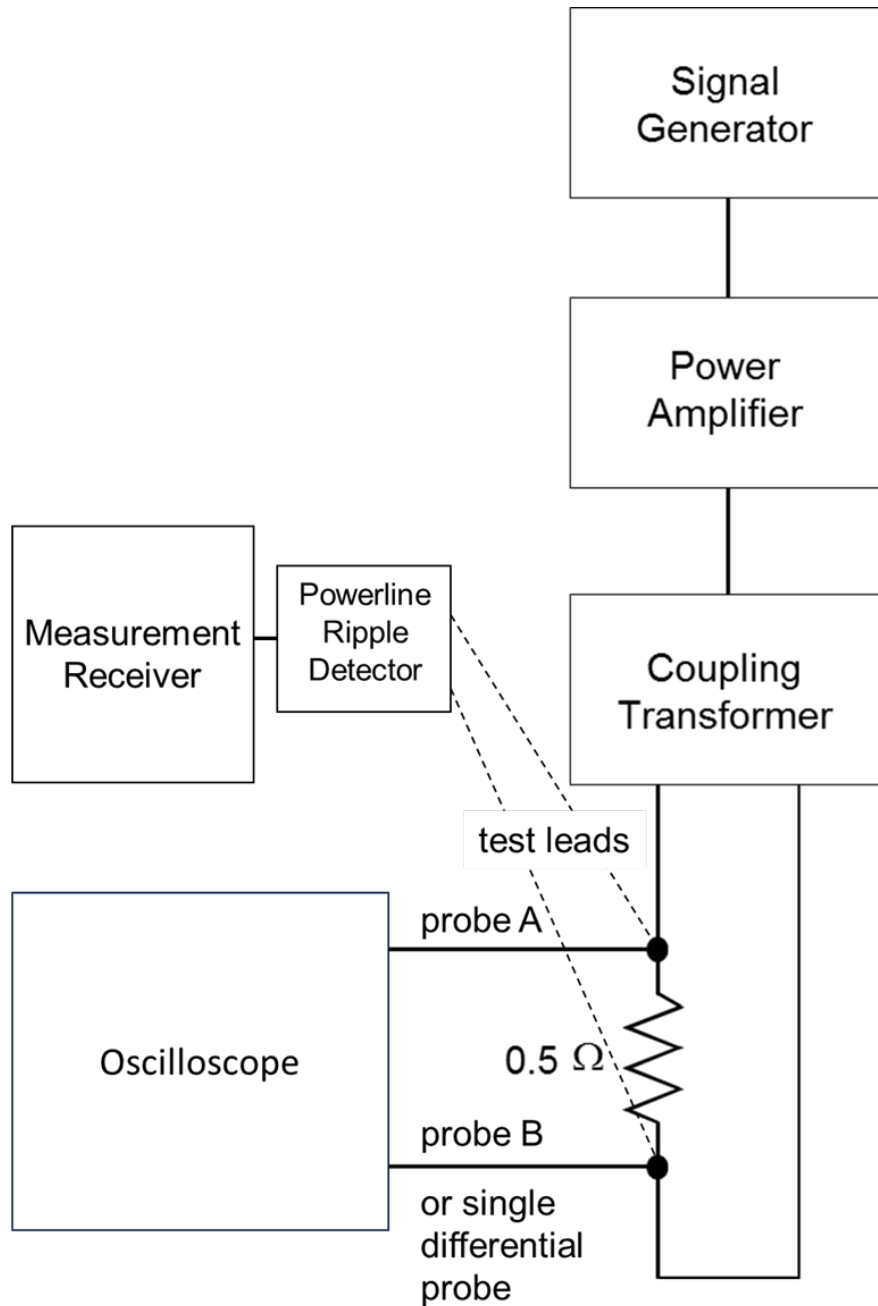
FIGURE CS101- 3. Calibration.
