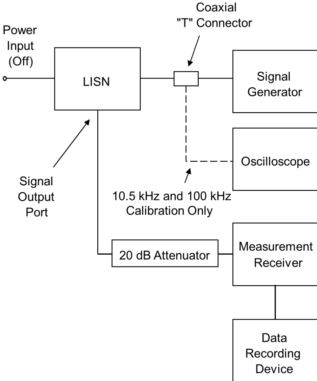
FIGURE CE102- 2. Measurement system check setup.
