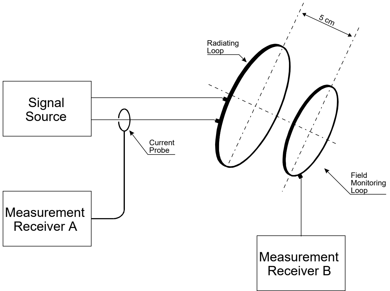
FIGURE RS101- 3. Calibration of the radiating system.
