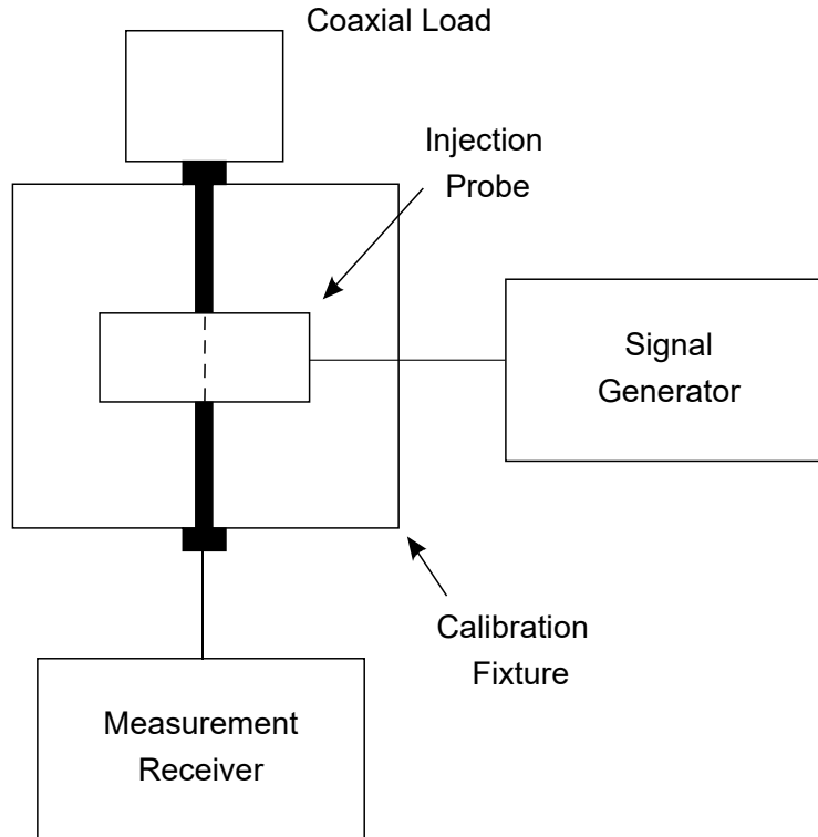
FIGURE A- 19. Insertion loss measurement.
