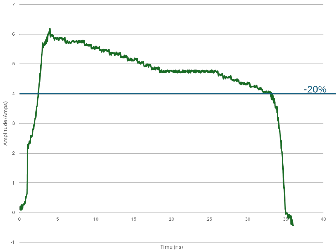
FIGURE A- 22. Typical CS115 calibration fixture waveform.
