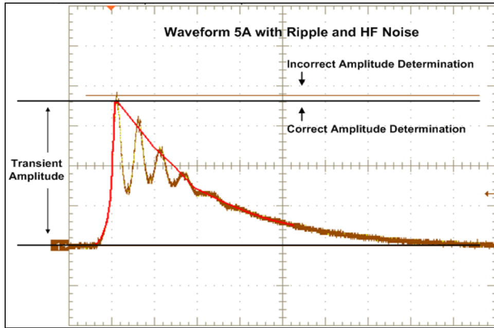
FIGURE A- 26. Ripple with high frequency noise - Waveform 5A amplitude determination.
