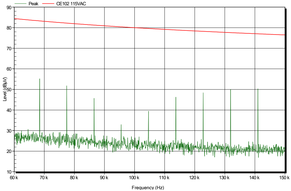
FIGURE A- 5. Traditional measurement receiver with 10 second scan time (minimum required by Table II ).
