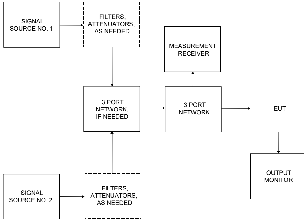
FIGURE A- 16. CS105 General test setup.
