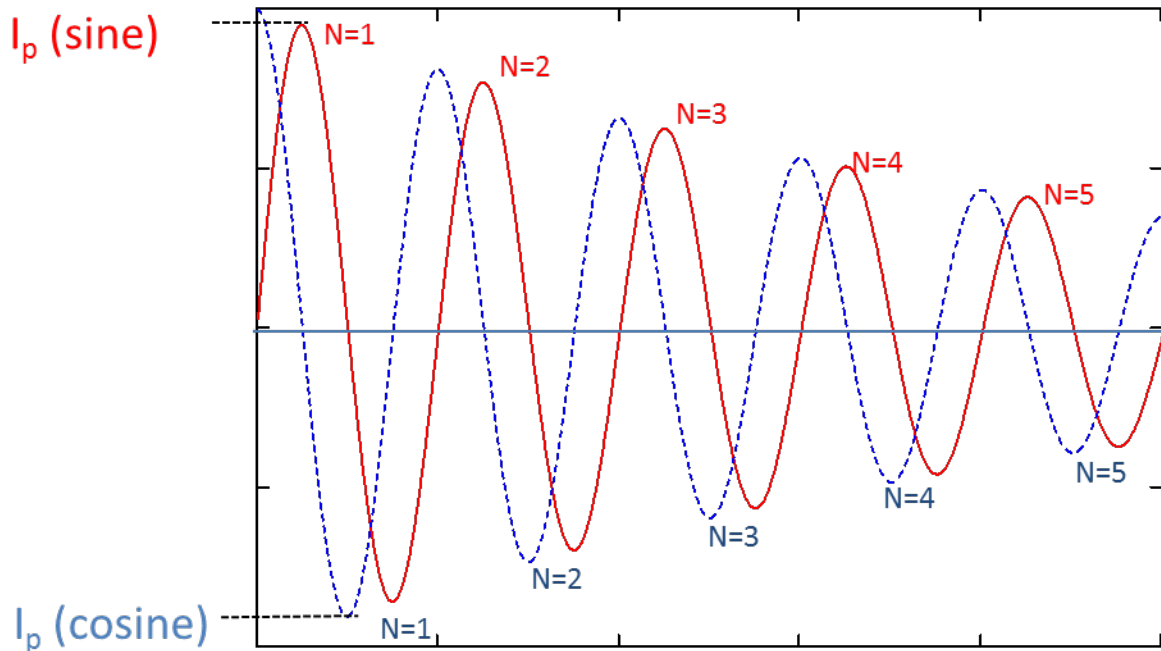
FIGURE A- 23. Typical CS116 calibration fixture sine and cosine waveforms.
