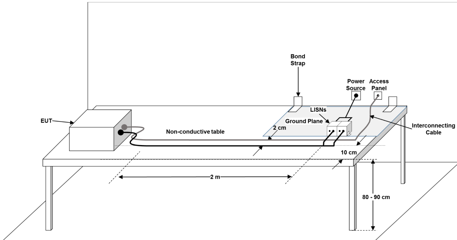
FIGURE 3. General test setup for non-conductive surface mounted EUT.
