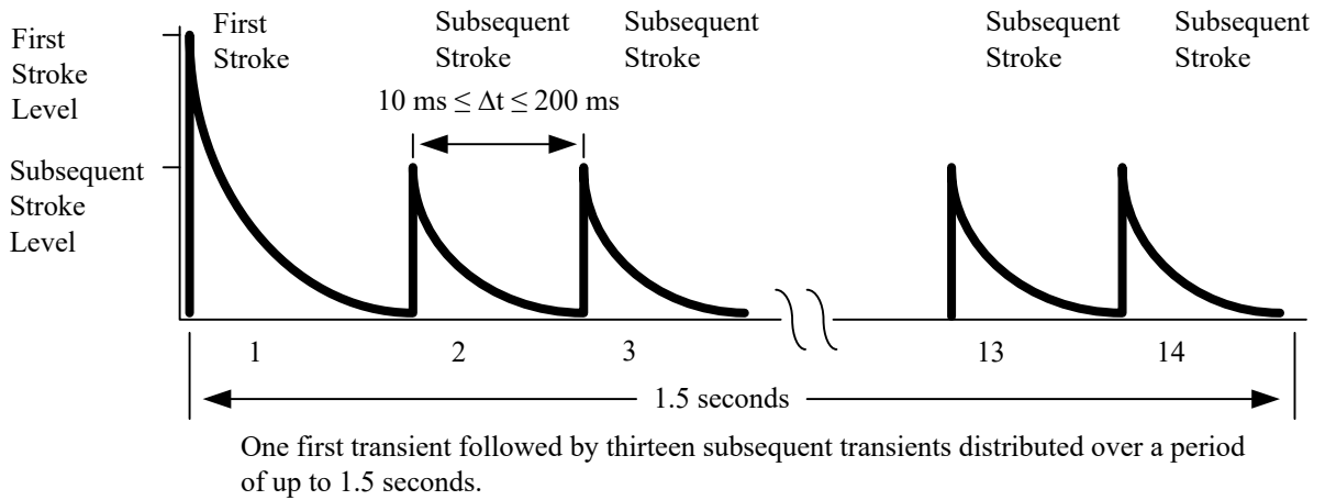
FIGURE CS117- 7. Multiple stroke application.
