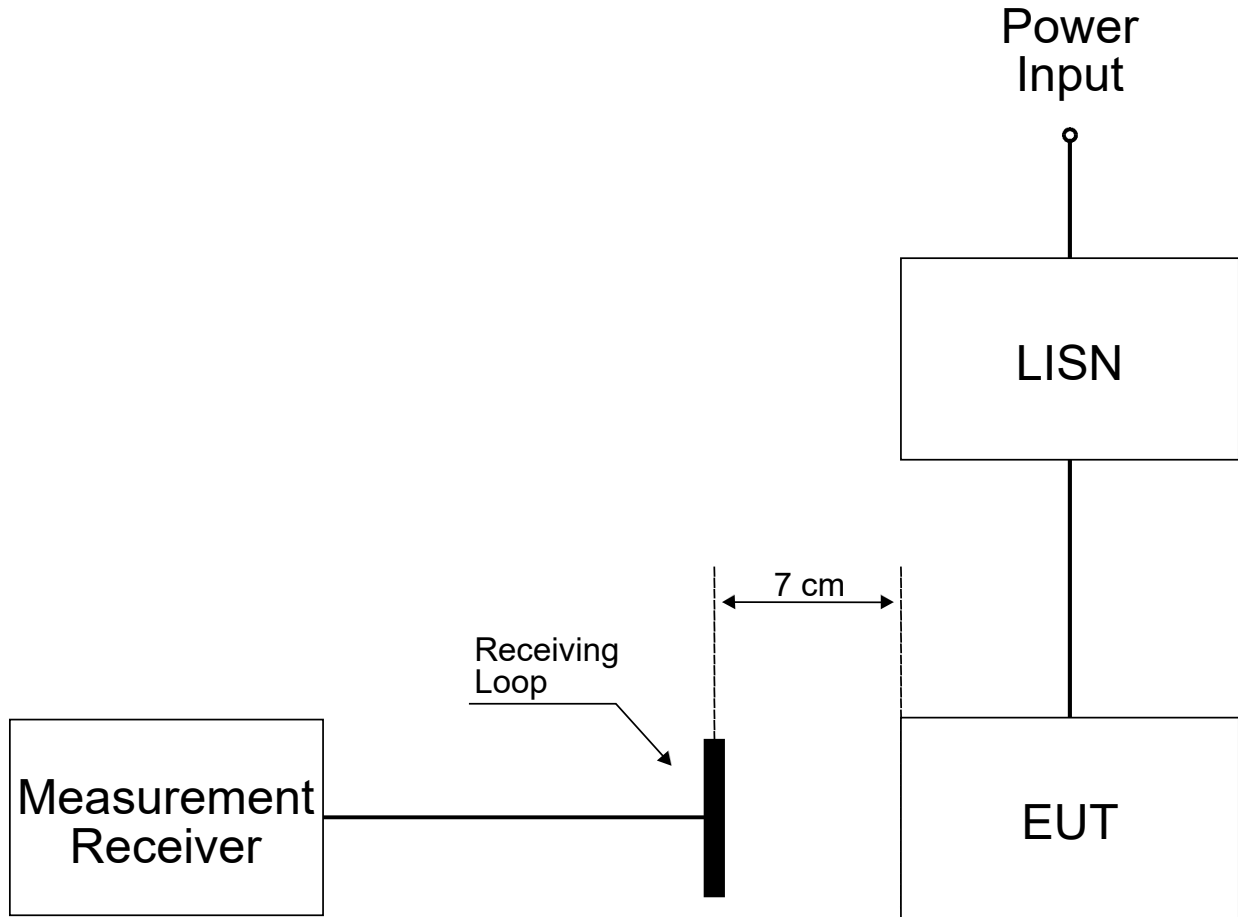
FIGURE RE101- 4. Basic test setup.
