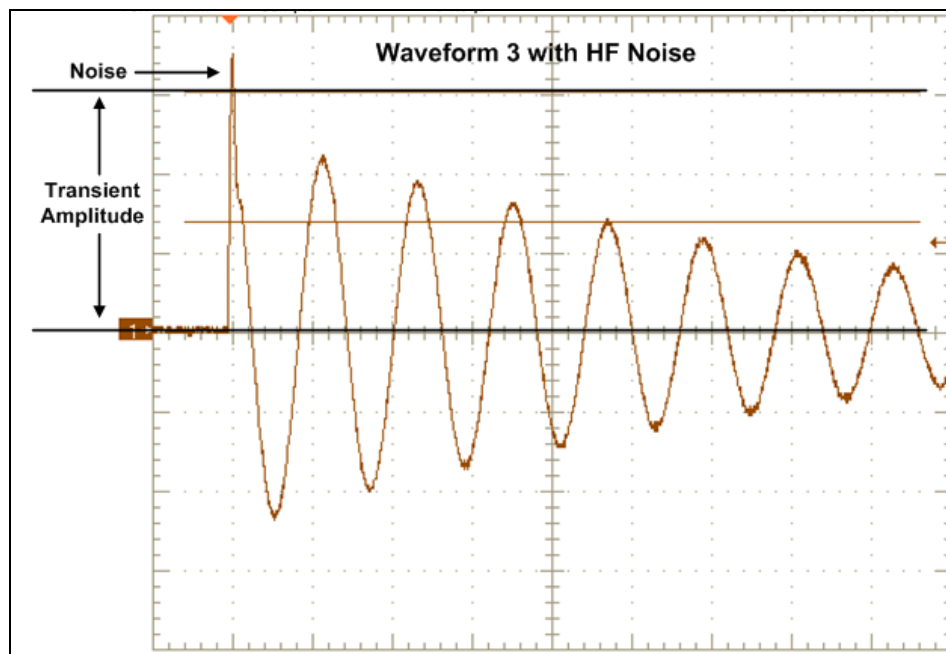
FIGURE A- 24. High frequency noise - Waveform 3 amplitude determination.
