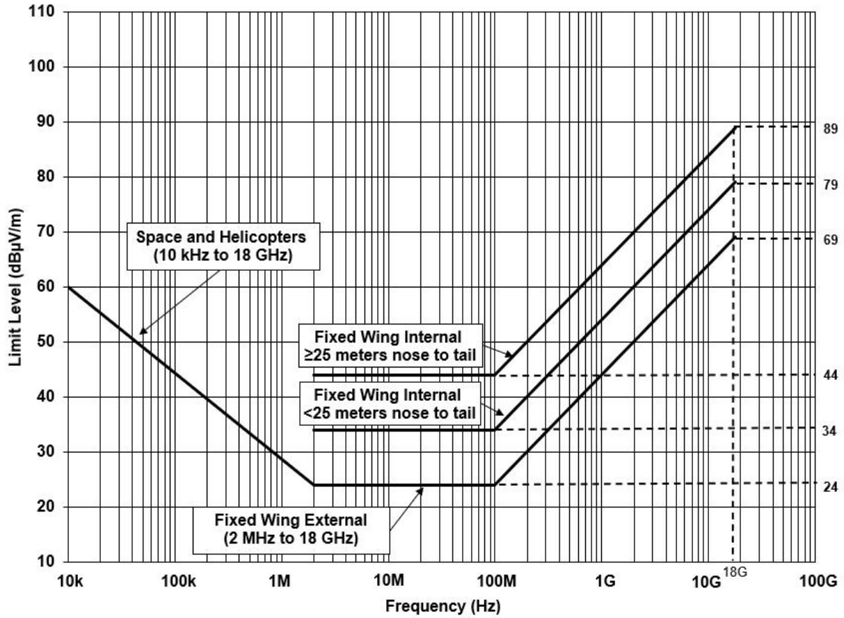
FIGURE RE102- 3. RE102 limit for aircraft and space system applications.
