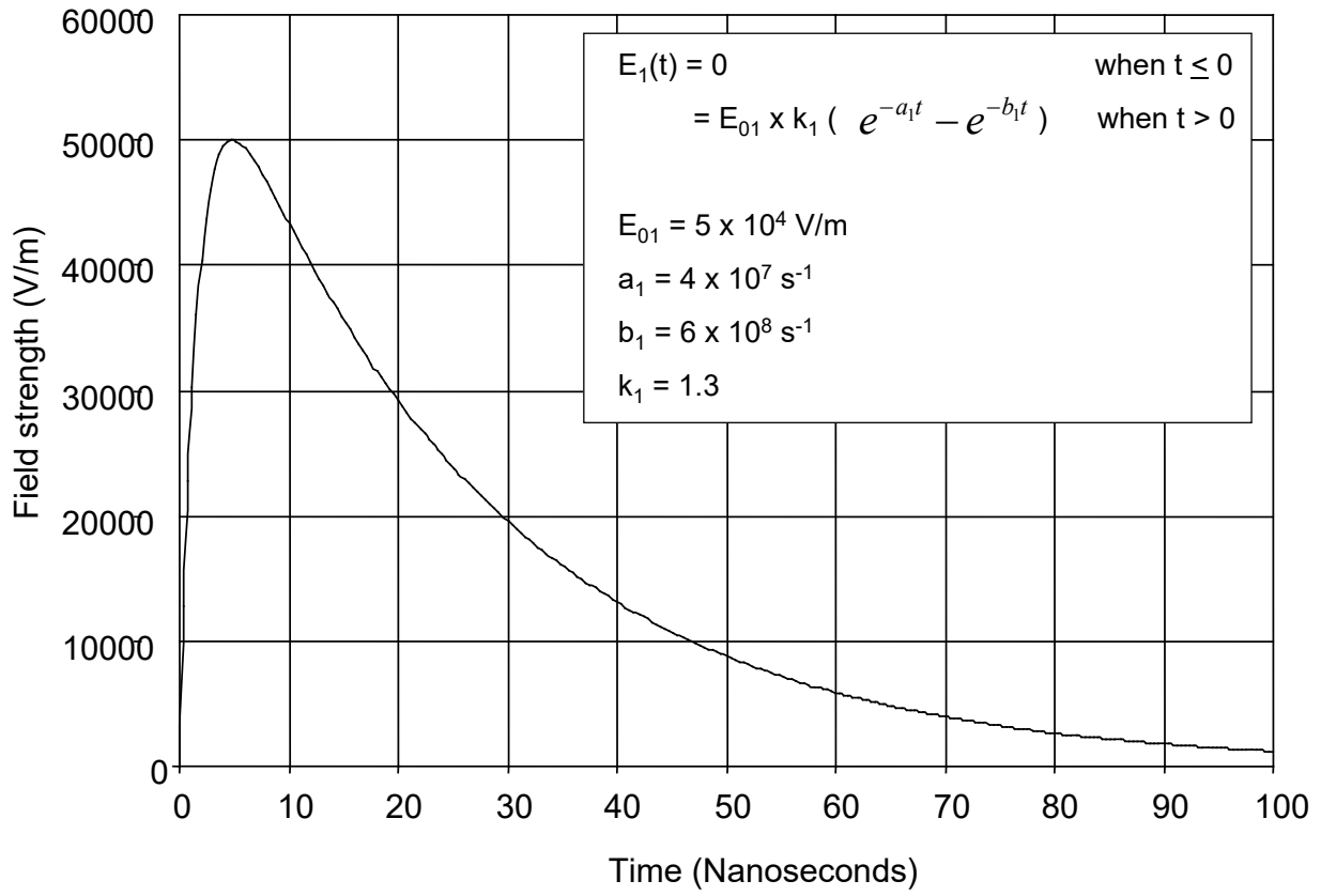
FIGURE RS105- 1. RS105 limit for all applications.
