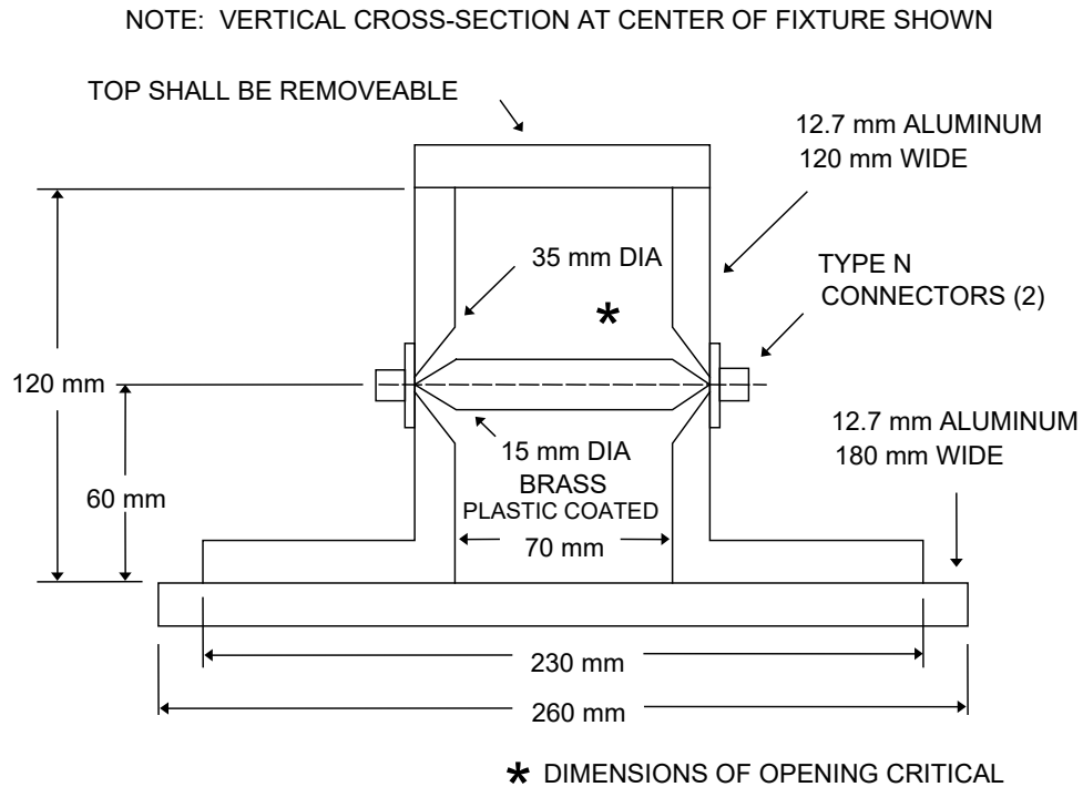
FIGURE A- 17. Typical CS114 calibration fixture.
