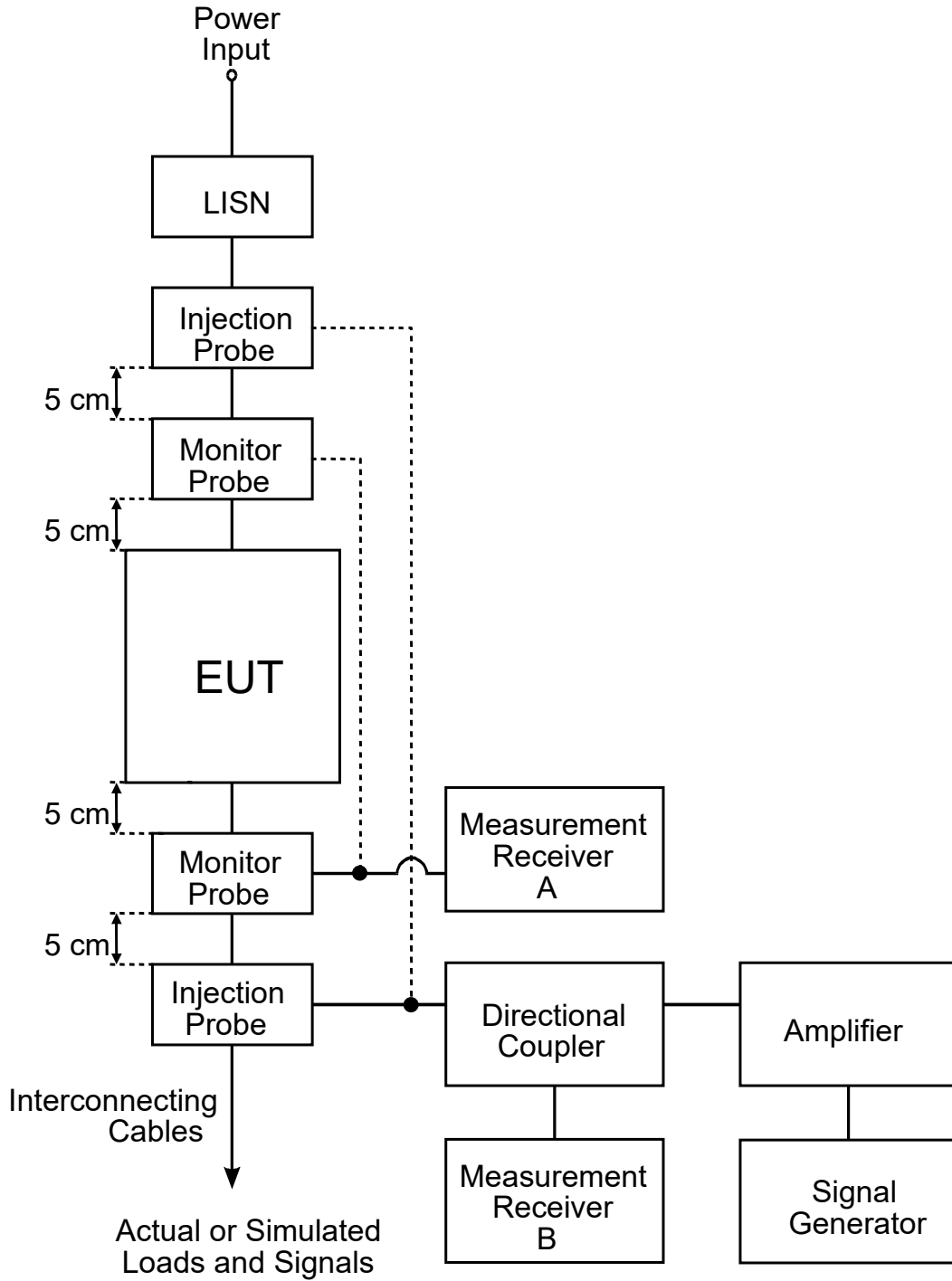
FIGURE CS114- 5. Bulk cable injection evaluation.
