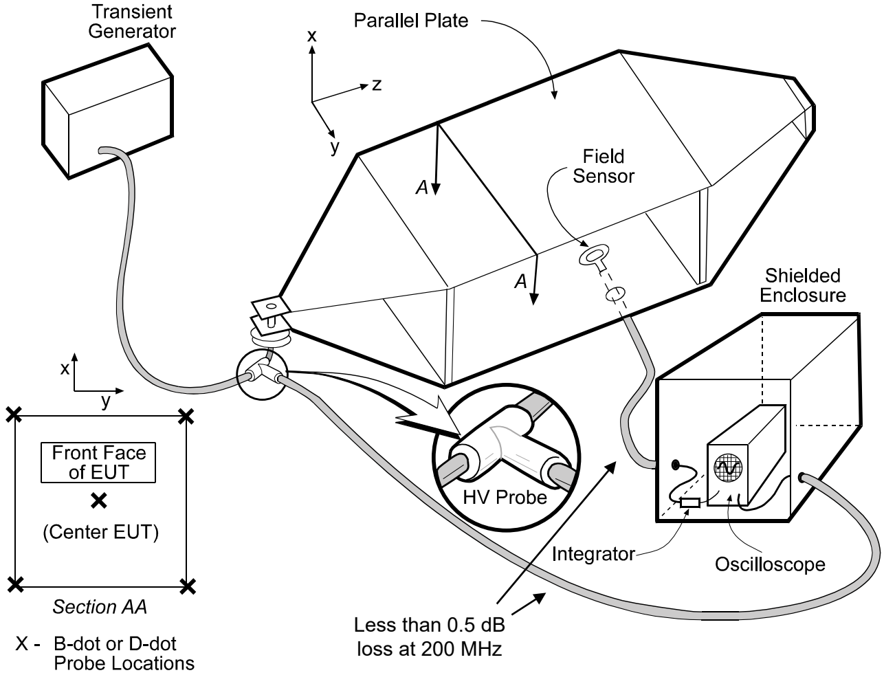
FIGURE RS105- 2. Typical calibration setup using parallel plate radiation system.
