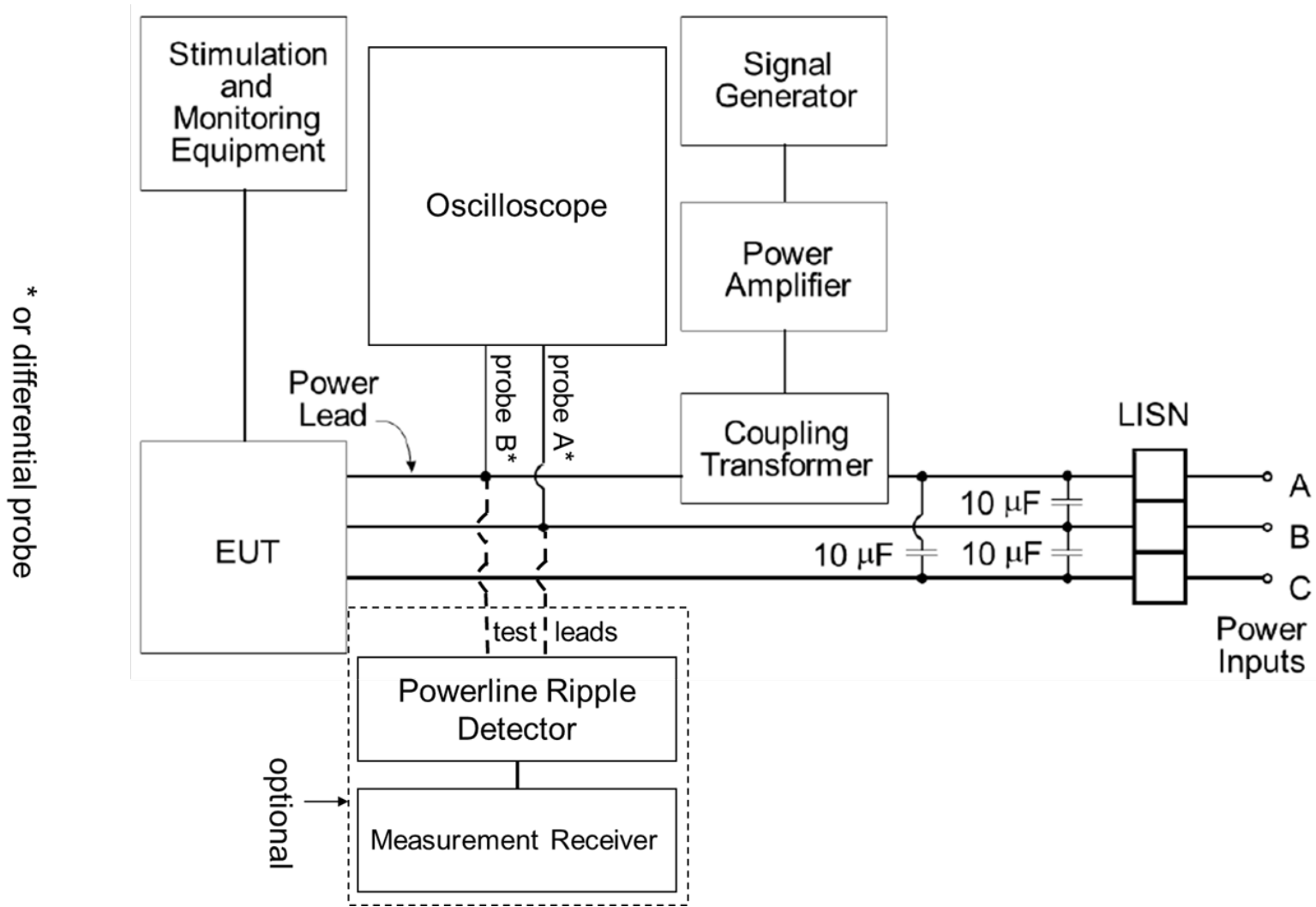
FIGURE CS101- 6. Signal injection, 3-phase delta.
