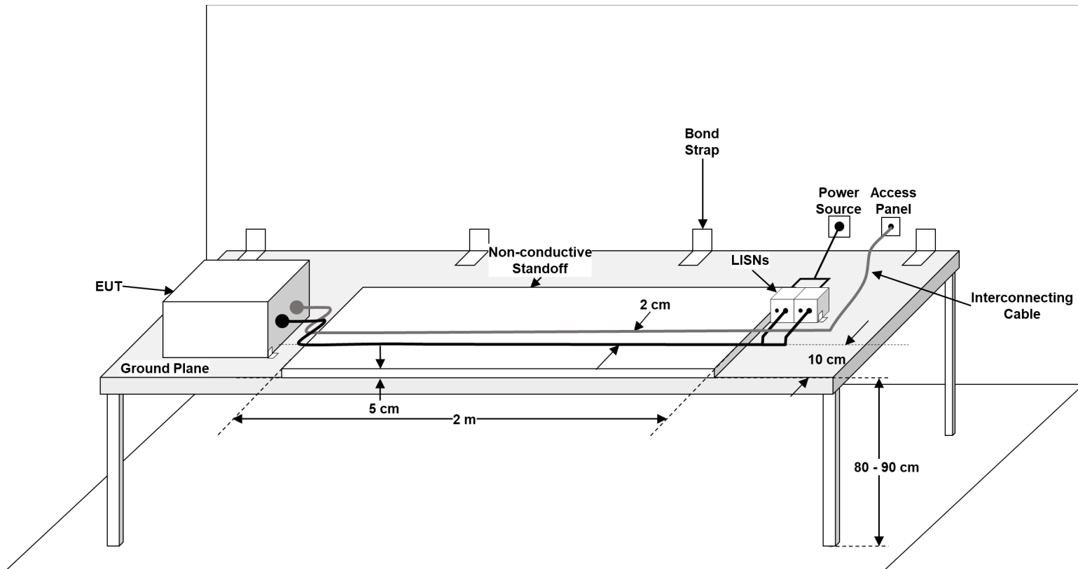
FIGURE 2. General test setup.
