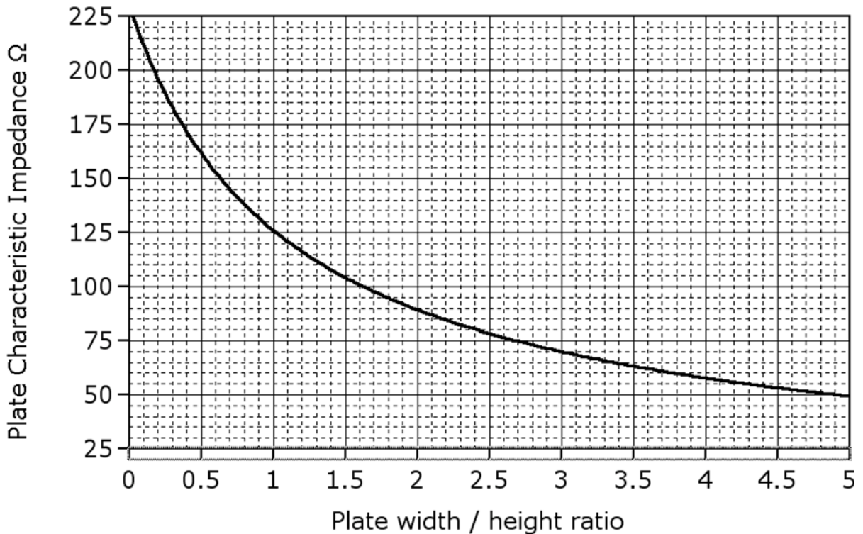
FIGURE A- 29. Plate characteristic impedance vs width-to-height ratio.
