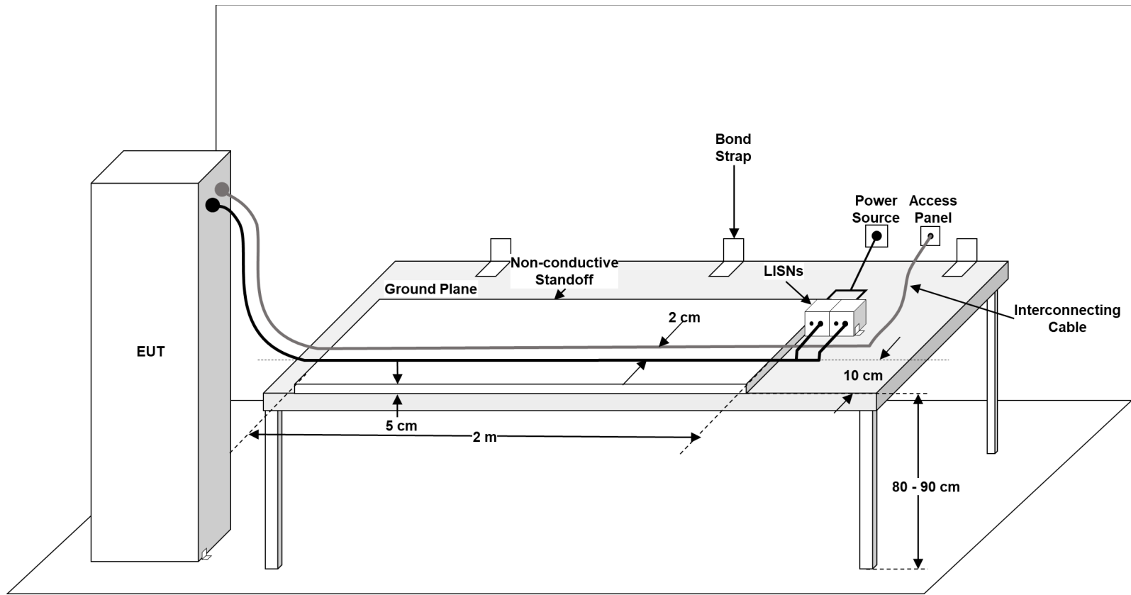
FIGURE 4. General test setup for free standing EUT in shielded enclosure.
