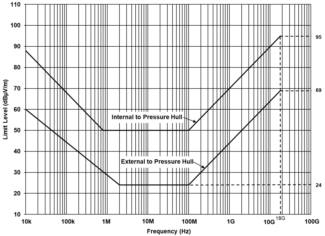
FIGURE RE102- 2. RE102 limit for submarine applications.
