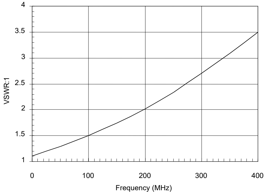
FIGURE A- 18. Maximum VSWR of calibration fixture.
