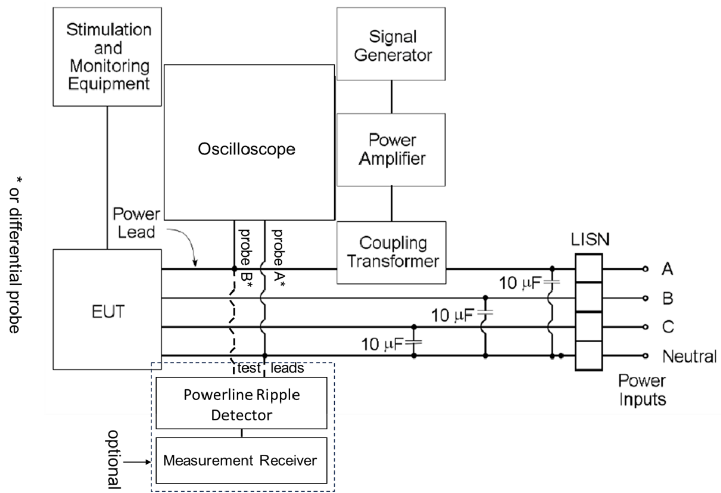
FIGURE CS101- 5. Signal injection, 3-phase wye.
