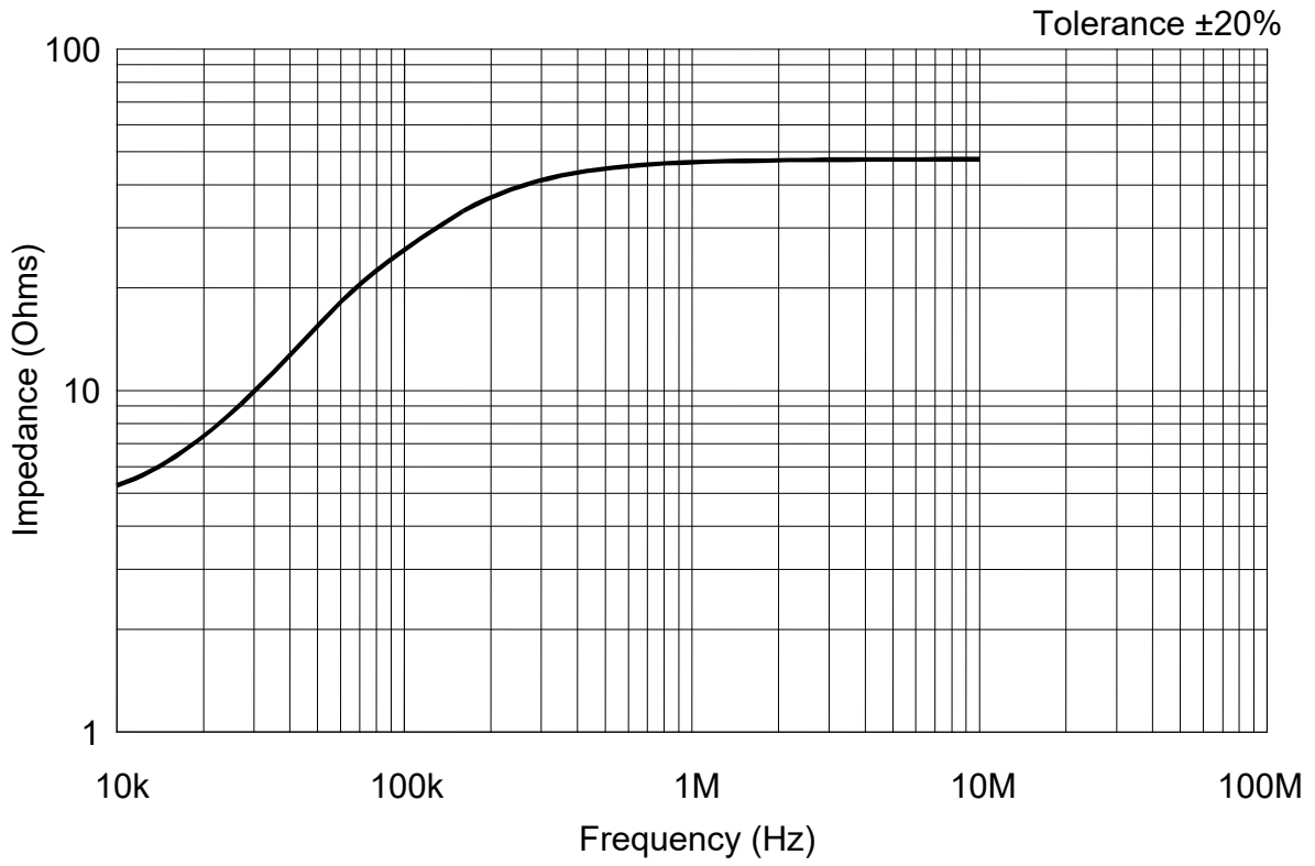
FIGURE 7. LISN impedance.
