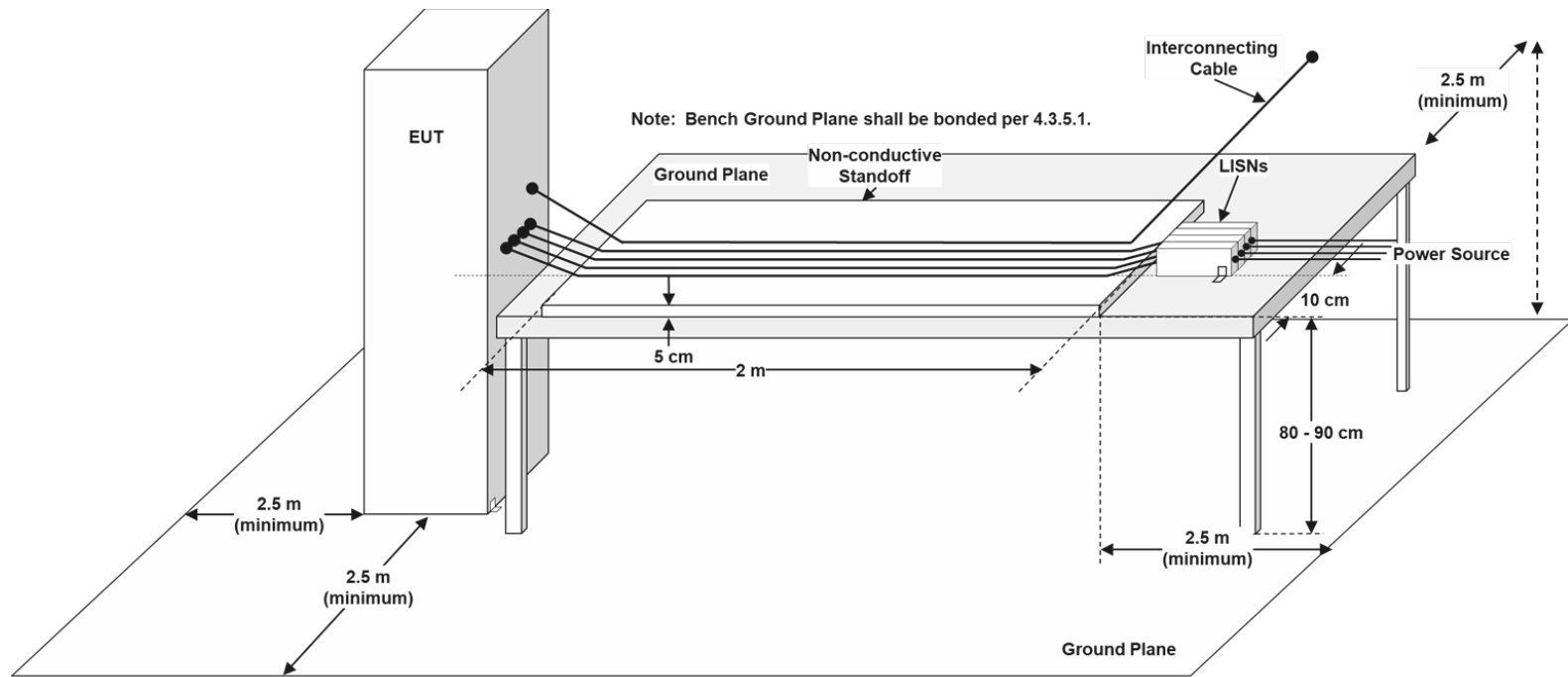
FIGURE 5. General test setup for free standing EUT outside shielded enclosure.
