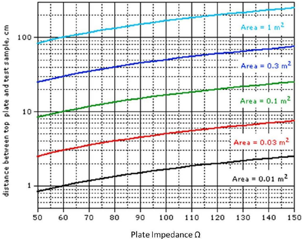
FIGURE A- 30. Required separation between top of test sample and top plate for various different plate constructions and test sample footprints.
