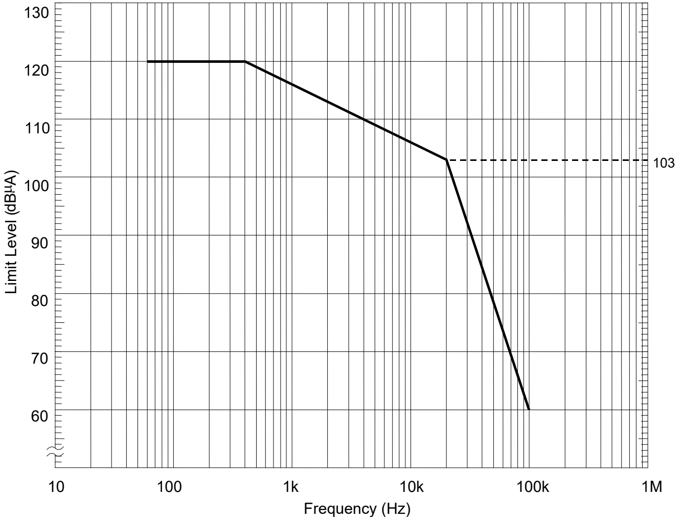
FIGURE CS109- 1. CS109 limit.
