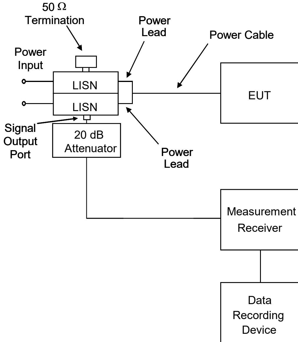
FIGURE CE102- 3. Measurement setup.
