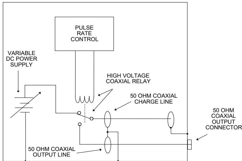
FIGURE A- 21. Circuit diagram of CS115 pulse generator.
