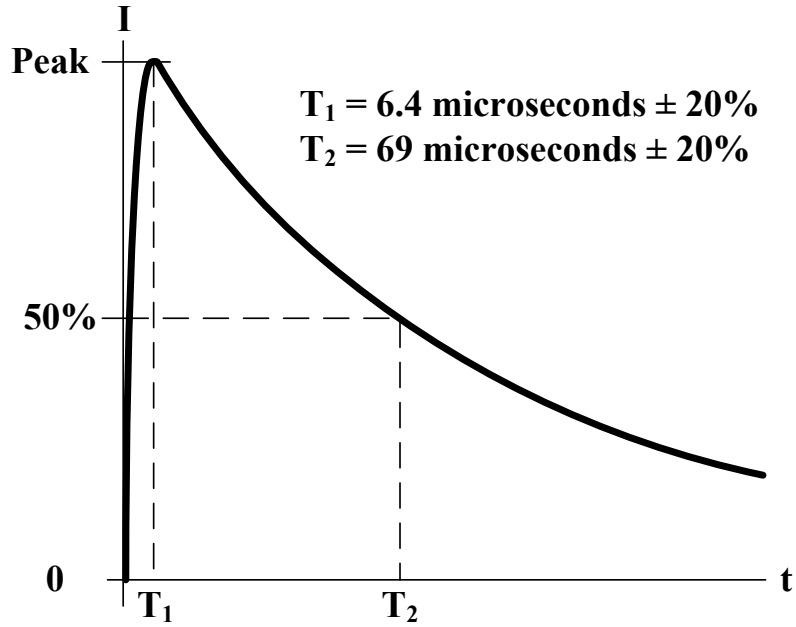
FIGURE CS117- 1. Current waveform 1.
