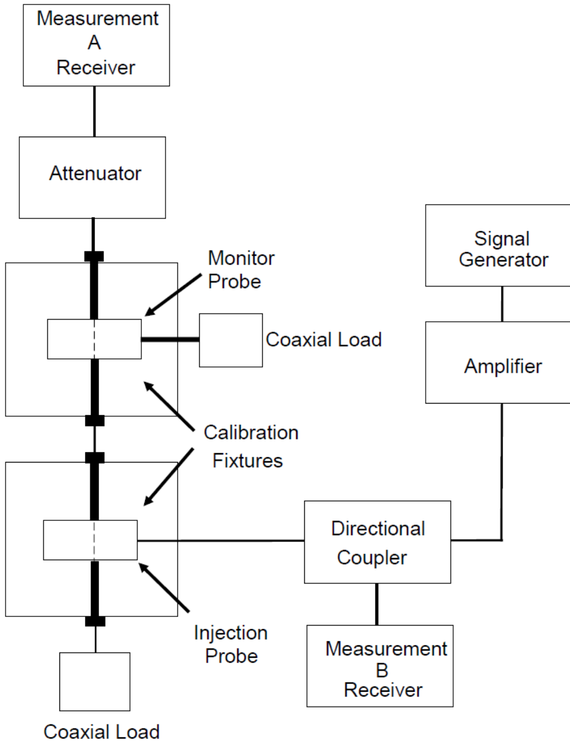
FIGURE CS114- 3. Calibration setup.
